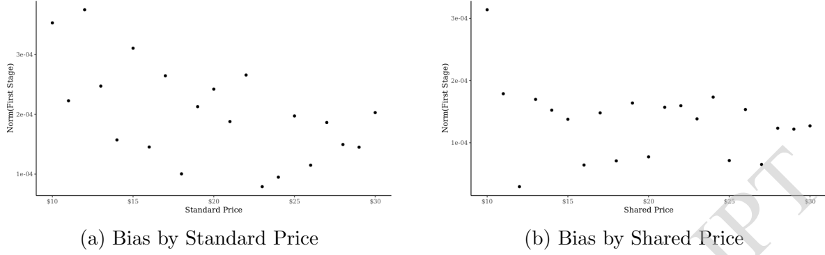
Figure A4: First Stage Bias in 2SLS
